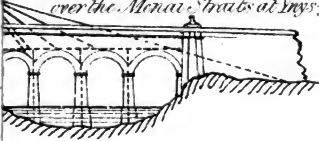
My first design for a Suspension Bridge over the Menai Straits at Ynys-y-Moch.
